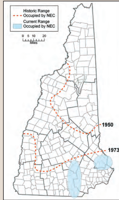
Historic range and remaining populations of New England cottontails
