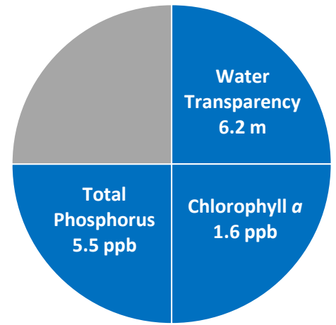
Figure 1. Crystal Lake Water Quality (2016)
