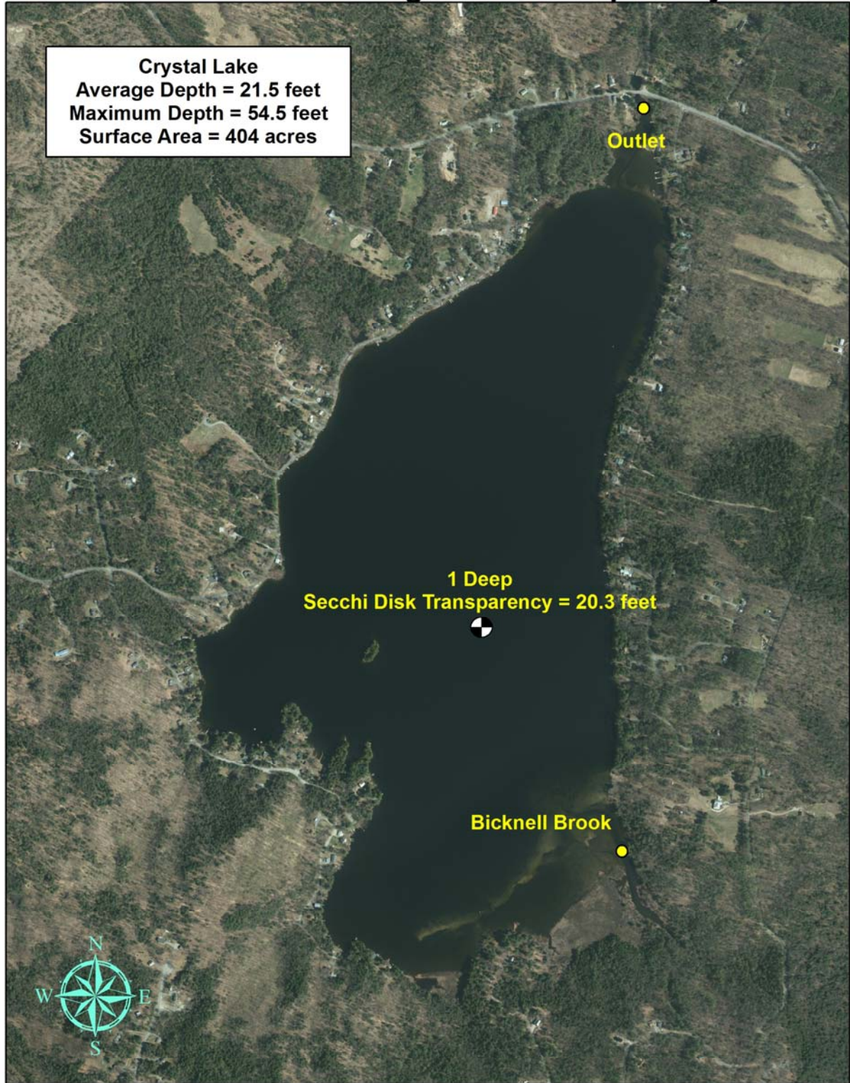
Figure 7. Crystal Lake (Enfield, NH) 2016 Deep and nearshore sampling locations and seasonal average water transparency
