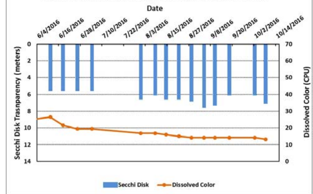
Figure 3. Crystal Lake - Site 1 Deep (2016 Seasonal Data) Secchi Disk Transparency and Dissolved Color Data
