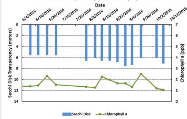
Figure 2. Crystal Lake - Site 1 Deep (2016 Seasonal Data) Secchi Disk Transparency and Chlorophyll a Data
