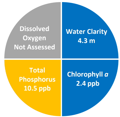
Figure 1. Naticook Lake Water Quality (2016)
