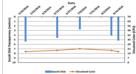
Figure 3. Naticook Lake - Site 1 Deep (2016 Seasonal Data) Secchi Disk Transparency and Dissolved Color Data
