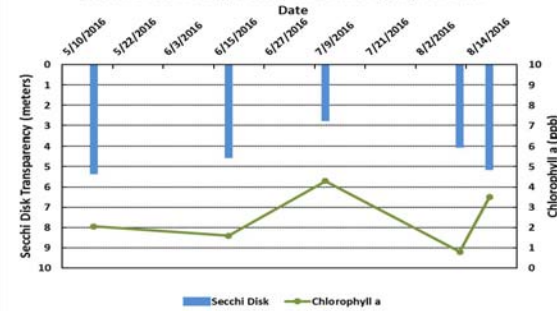
Figure 2. Naticook Lake - Site 1 Deep (2016 Seasonal Data) Secchi Disk Transparency and Chlorophyll a Data
