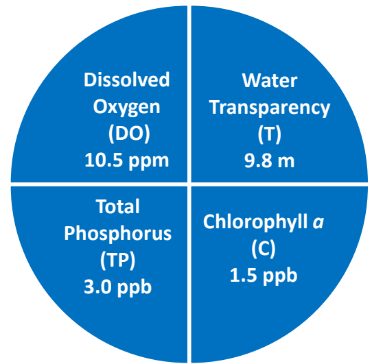
Figure 1. Station Deep 1 Water Quality (2017)
