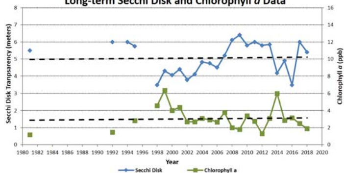
Figure 4. Ivanhoe - Site 2 Ivanhoe (1981-2018) Long-term Secchi Disk and Chlorophyll a Data
