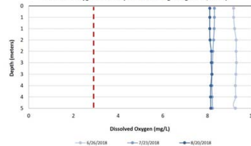
Figure 6. Lake Ivanhoe - Station 1 Deep Dissolved Oxygen Profiles (June 26 through August 20, 2018)
