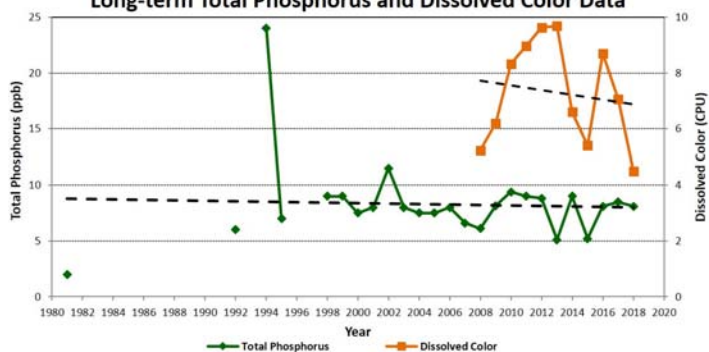
Figure 5. Ivanhoe - Site 2 Ivanhoe (1981-2018) Long-term Total Phosphorus and Dissolved Color Data
