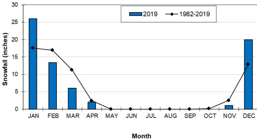
Monthly Snowfall (1982-2019)
