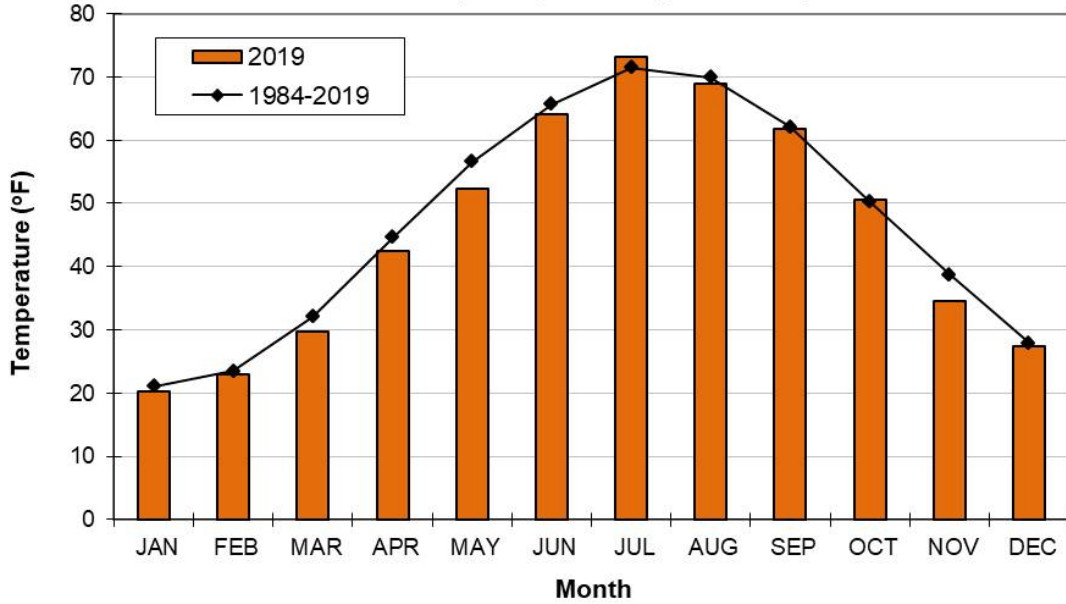
Monthly Temperature (1984-2019)
