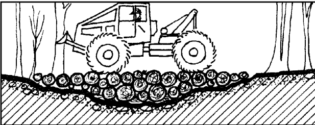
LOG OR POLE FORD — minimum 8"-10" diameter poles or cull logs side by side — protect bank and channel — use well casing to maintain water flow — remove at closeout
